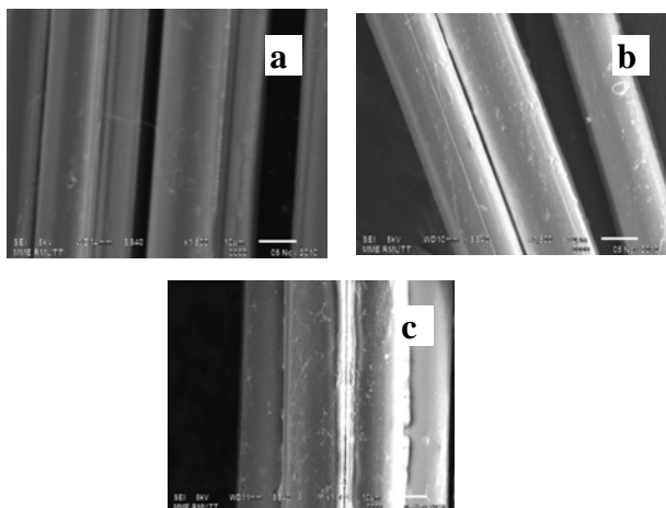
Fig. 3 SEM images of PLA/PHBV blends: (a) 100/0, (b) 95/5, (c) 85/15.
