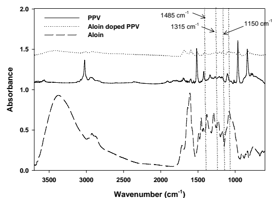
Figure 1 Absorption infrared spectra of: poly(p-phenylene vinylene), PPV; Aloin; and Aloin doped poly(p-phenylene vinylene), Aloin doped PPV.
