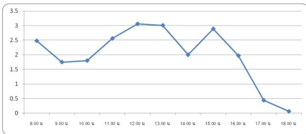
Figure 11. AC current of the grid connected inverter
