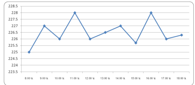
Figure 14. Average AC voltage of the inverter
