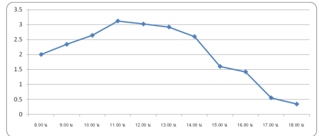
Figure 13. Average DC current of PV panel
