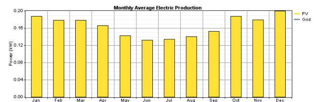
Figure 2. Power output of PVside
