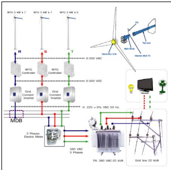
Fig. 3 schematic diagram of 100 Kw mini wind farm located in Thayang, Pecthaburi Thailand
