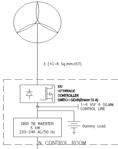
Fig.2 One Unit of 5 KW wind turbine system configuration
