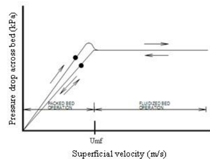
Fig.1. Relationship between pressure drop across the bed with fluid velocity
