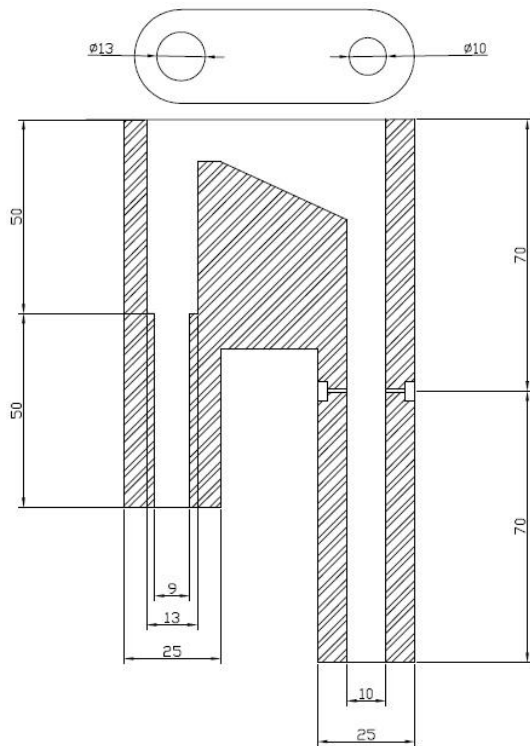
Fig.2. design drawing of the two-stage gasifier
