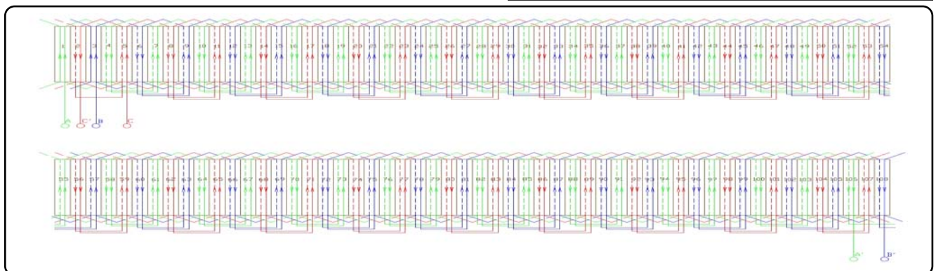
Fig. 5. Winding Diagram
