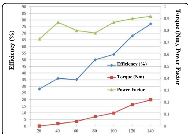
(b) speed comparison with torque, efficiency and p.f.
