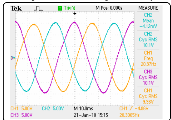
(a) 3 Phase Voltage Waveform
