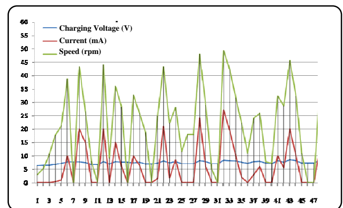
Fig. 18. Charging voltage, current and speed
