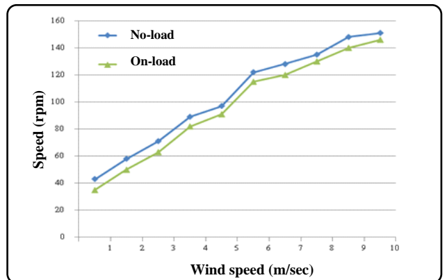
Fig. 15. Comparison roof ventilator when no-load and on-load that effect to speed
