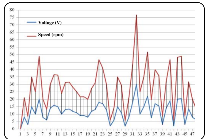
Fig. 17. Voltage and Speed at no-load
