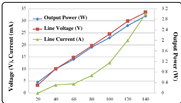
(a) Speed comparison with voltage, current and power
