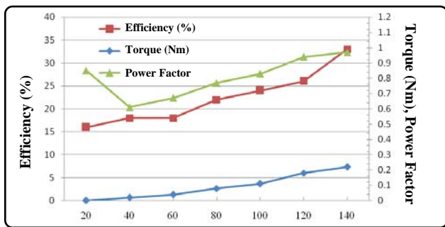
(b) speed comparison with torque, efficiency and p.f.
