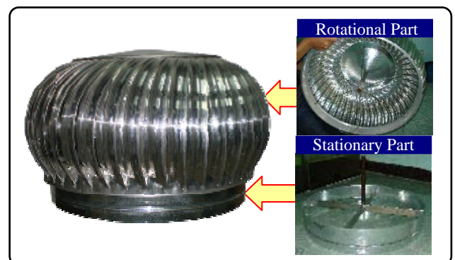
Fig.2. Construction of Roof Ventilator
