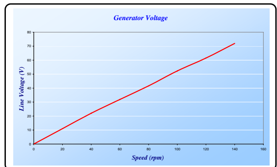
(b) Plot Curve between Speed and Line Voltage Fig. 11. Voltage measurement from generator
