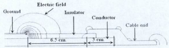
Fig 3 Contour of Electric Field at the tip of cable line
