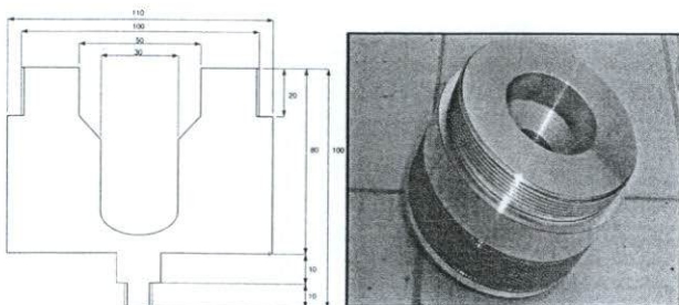
Fig. 6: Show the pattern and the base supporter for the high voltage cable terminator
