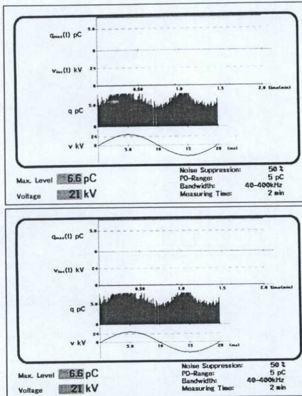
Fig 11: Show the example of the testing in the Partial Discharge Model
