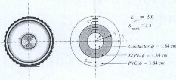
Fig. 2 Showing the structure in the period that has the electric field stress in the high voltage cable XLPE
