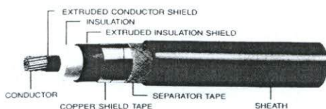
Fig. 1 Structure inside the High Voltage Cable
