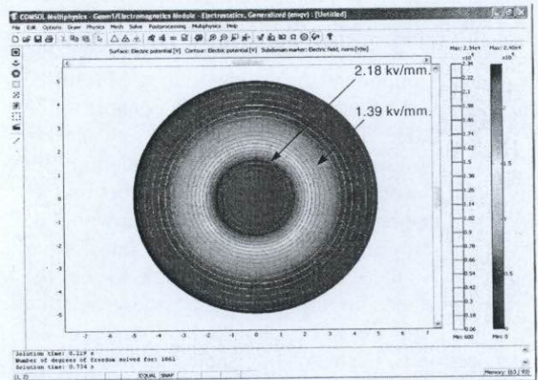
Fig 4 Show Simulations Electric Field Analysis
