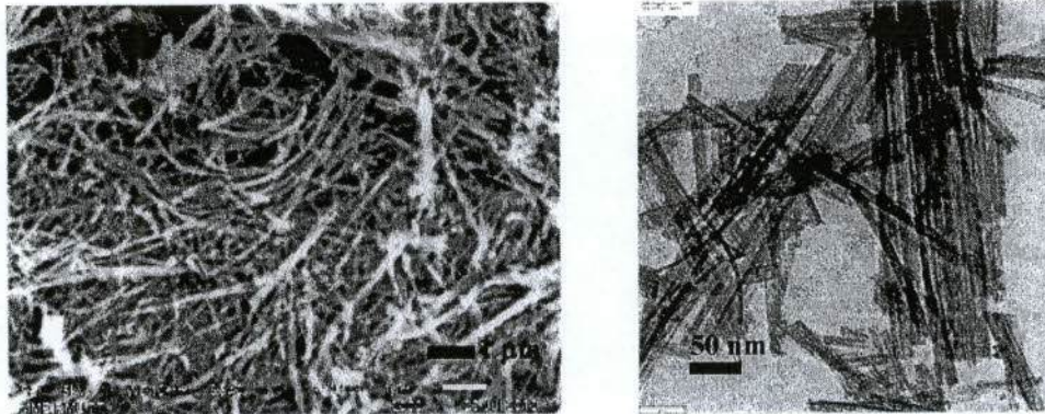
Fig. 1. (a) SEM image (b) TEM image of the as-synthesized sample at 115^\circ\text{C} for 24 h.
